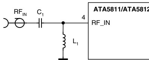
Figure 7. Input Matching to 50 \Omega
