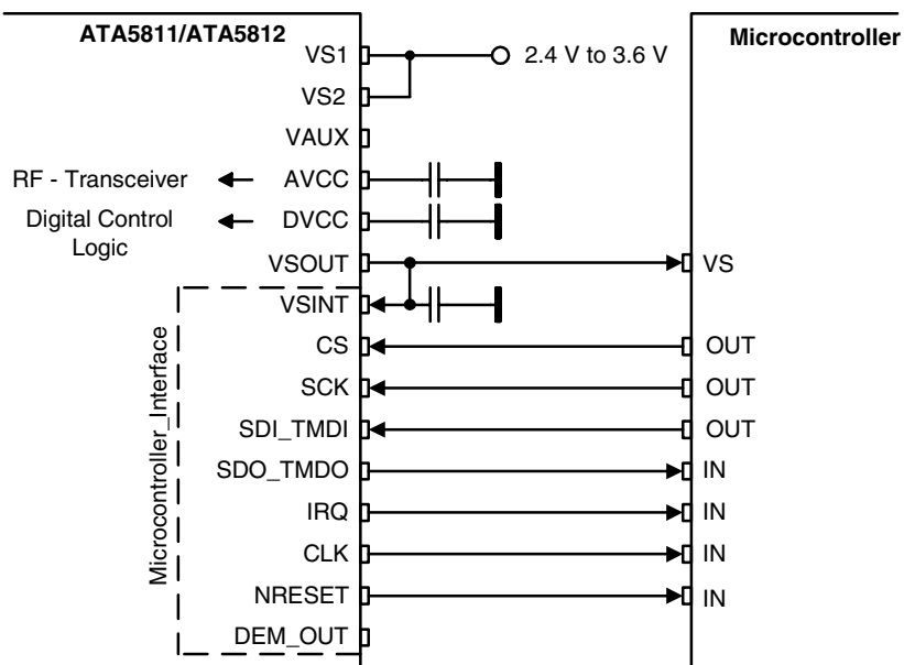
Figure 25. 1-Battery Application
